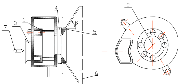
FIG 6. Scheme of the frontal device No. 2: 1 – air swirler of the central zone; 2 – centrifugal fuel nozzle of the first contour; 3 – air intake of the central zone; 4 – air swirler of the second contour; 5 – conical outlet; 6 – cylindrical outlet; 7 – jet fuel nozzle of the second contour
