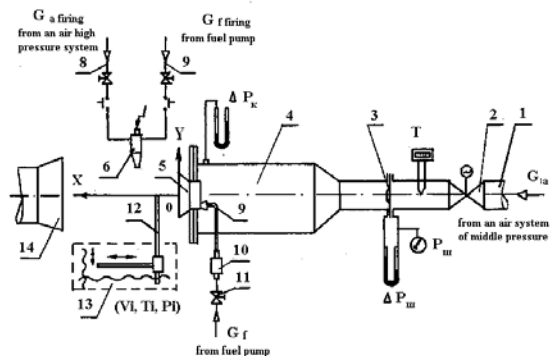
FIG 5. The scheme experimental installation:
