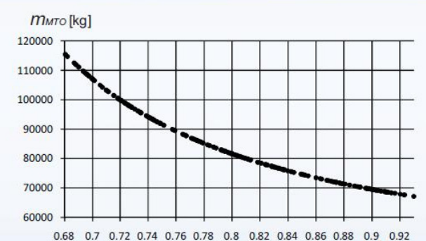
Fig. 4 Maximum take-off mass, m_{MTO} as a function of the maximum landing mass ratio, m_{ML}/m_{MTO}
