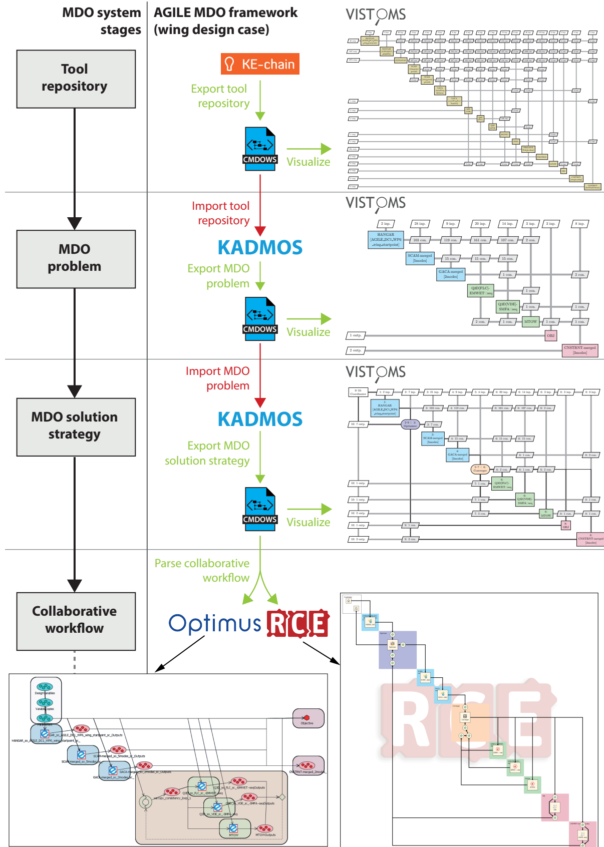
Figure 14: Visualization of the AGILE MDO framework applications from Fig. 13 for the wing design case, mapped on the first four stages of the MDO system in Fig. 1
