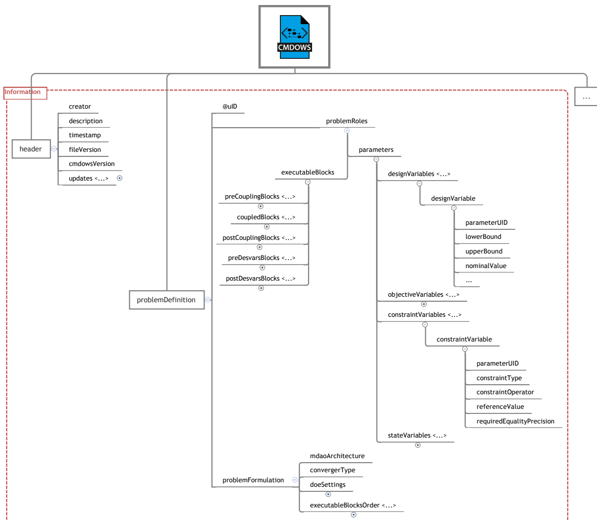
Figure 7: Elements in the CMDOWS category Information
