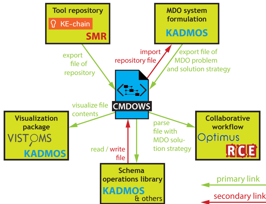
Figure 13: The established links between CMDOWS and the AGILE MDO framework applications for the wing design case study
