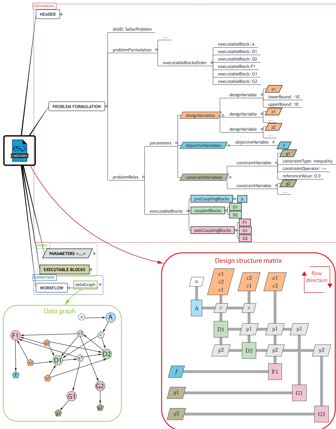
Figure 11: Illustration of the storage of the Sellar MDO problem in a CMDOWS file
