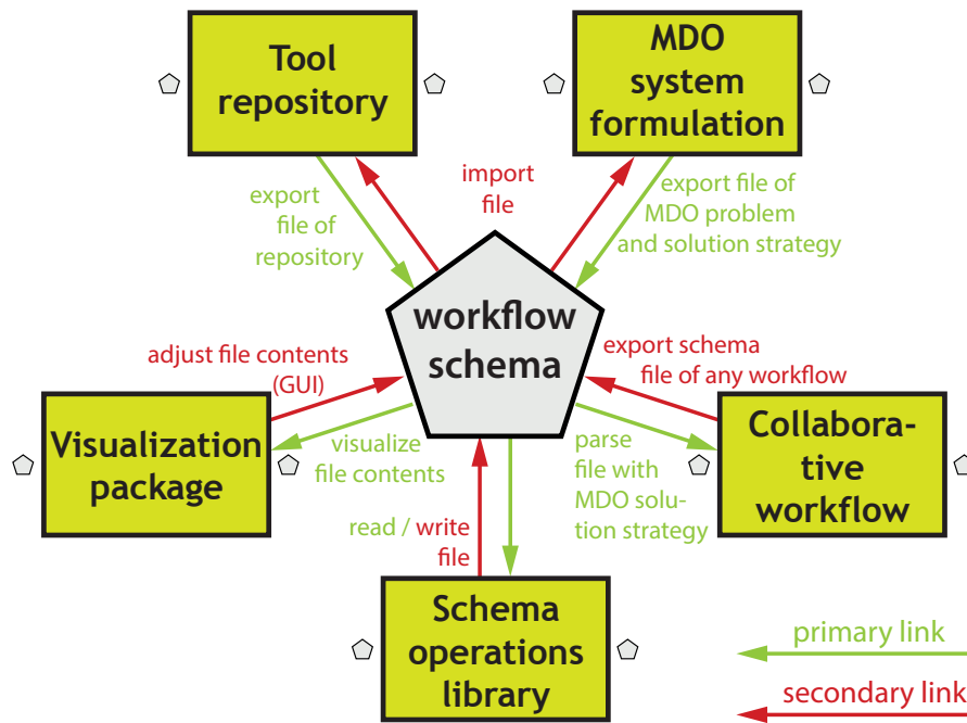
Figure 5: Primary and secondary links between the workflow schema and the MDO framework application categories
