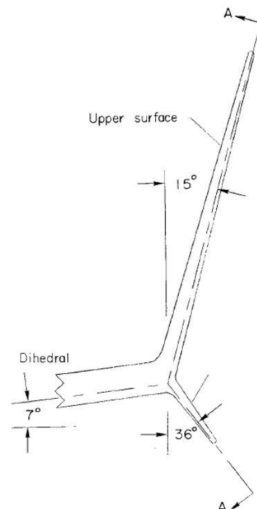
Figure 4: Whitcomb's winglet [17]
