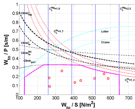
Figure 2: Sizing matrix plot for the considered motor-glider
