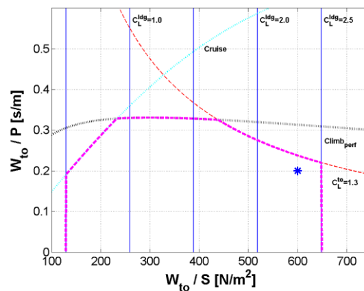
Figure 5: Sizing matrix plot with selection of the design point
