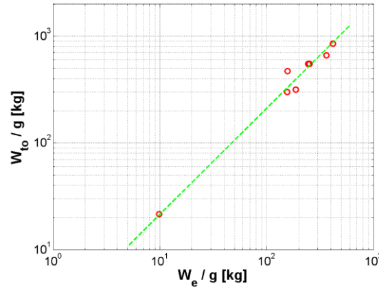
Figure 1: Real weight data and statistical regression for the considered database
