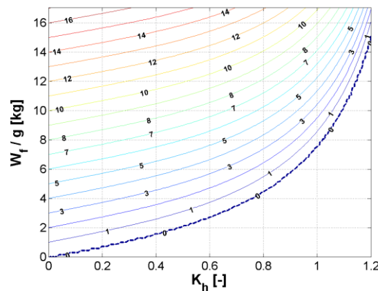
Figure 10: Contour plot of residual fuel weight at the end of the cruise as a function of W_f and K_h
