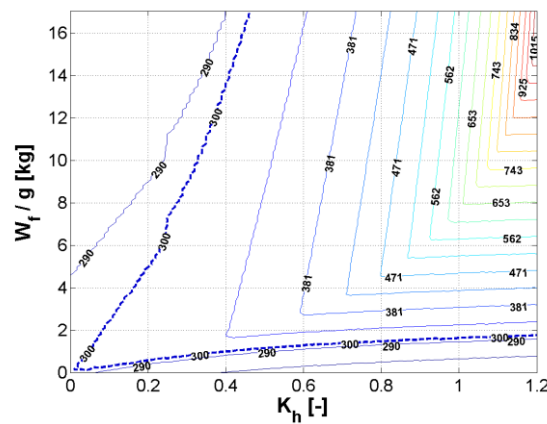
Figure 9: Contour plot of cruising range as a function of W_f and K_h
