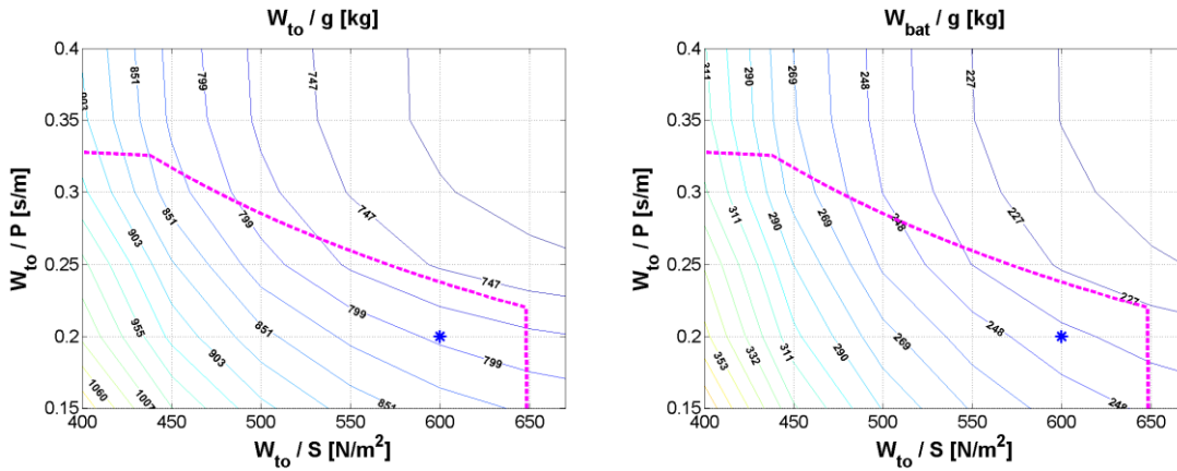
Figure 7: Effect of a change in the design point on weights
