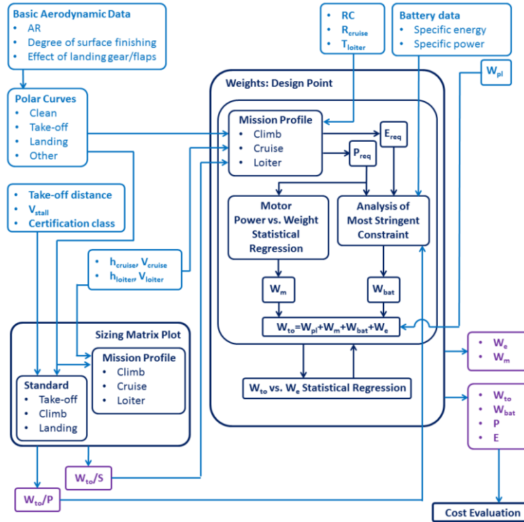
Figure 3 Integrated preliminary design workflow
