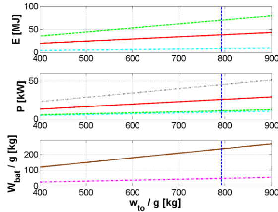
Figure 6: Battery energy, power and weight as functions of W_{to}
