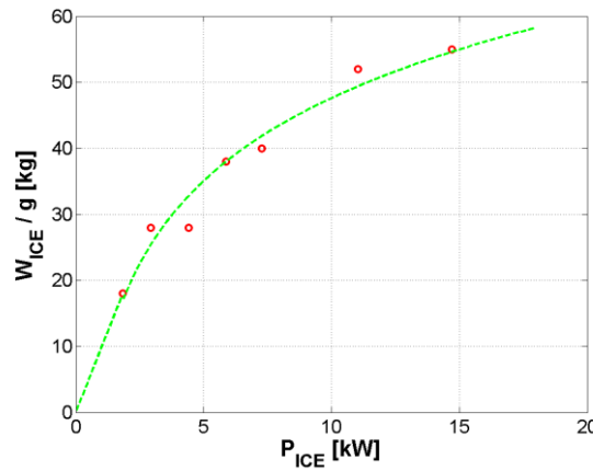
Figure 4: Database and analytical fitting of ICE power plants for a hybrid electric propulsion system
