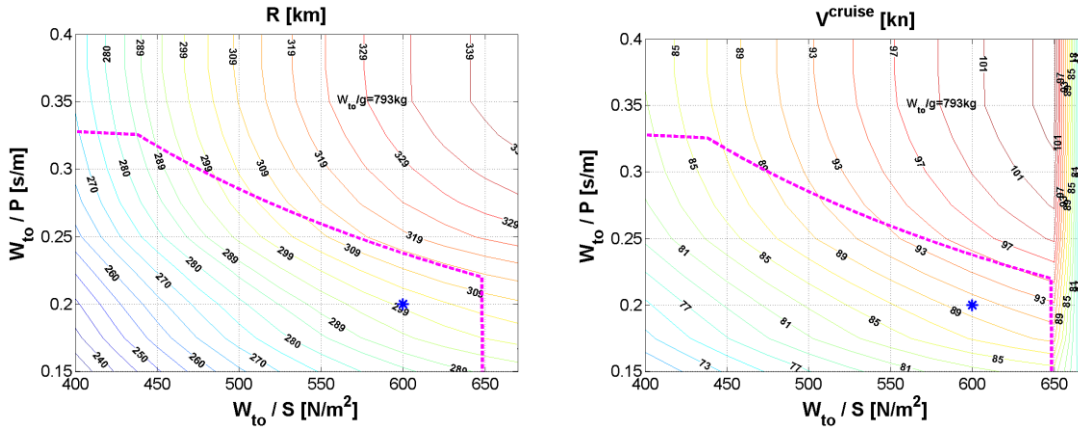
Figure 8: Effects of a change in the design point on performance (fixed weights)
