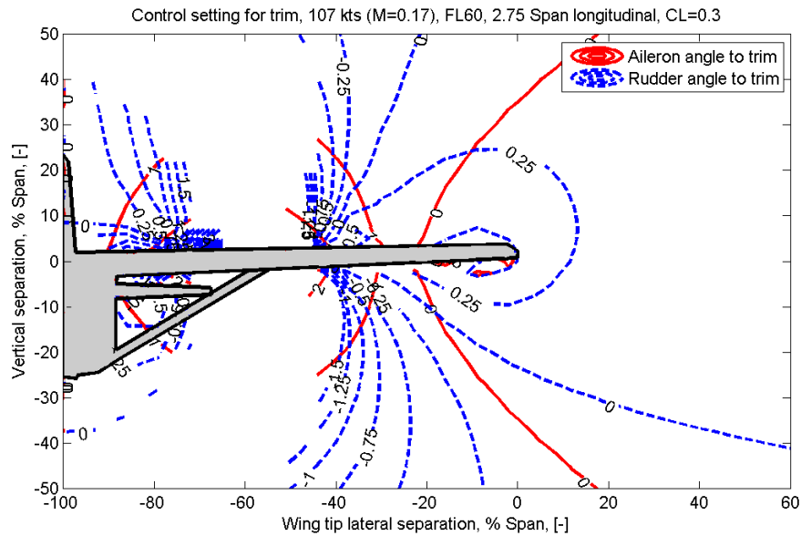
Fig. 7: Iso curves of control surface deflection to trim.
