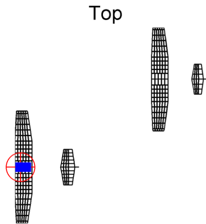
Fig. 4: Mesh setup for the Cessna formation, top view. C182 as lead aircraft, C152 as number 2. The longitudinal separation is 2.75 span
