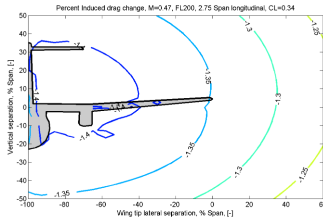
Fig. 12: Iso curves of induced drag reduction of the lead aircraft, showing the Bombardier Dash-8 outline.
