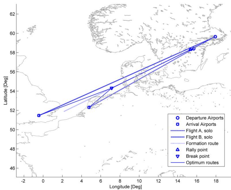
Fig. 13: Flight routes between LPI - AMS and ARN – LHR, Together with the optimized formation route
