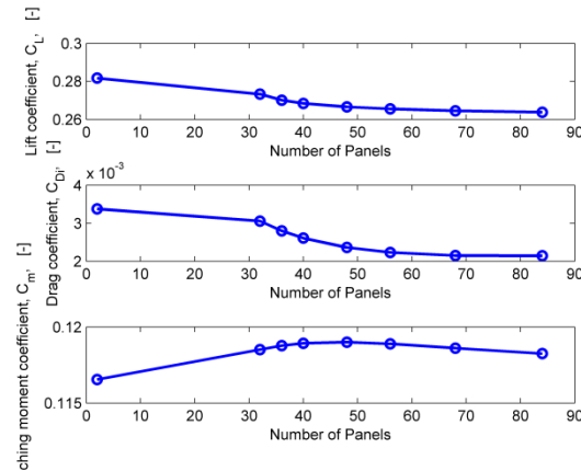
Fig. 5. Grid convergence study for the Cessna geometries.
