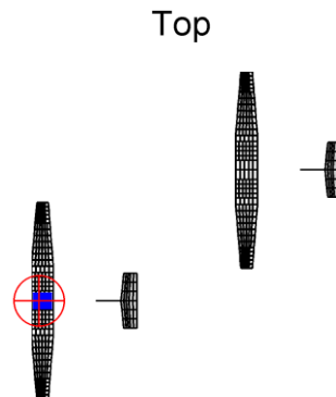
Fig. 8: Numerical mesh for the commercial Dash-8 formation case, top view. The following aircraft in position [2.75 0 -1], [Span].
