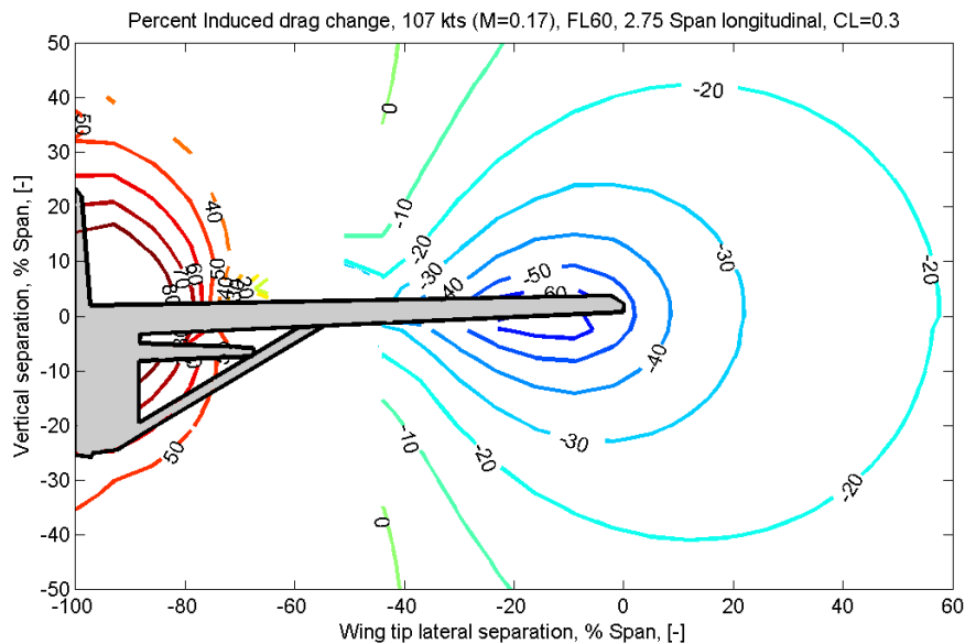
Fig. 6: Iso curves of induced drag reduction in percent of the following aircraft, showing the Cessna 182 outline. Origin position marks wingtip to wingtip
