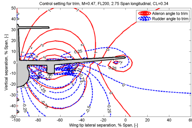
Fig. 11: Iso curves of control surface deflection to trim.
