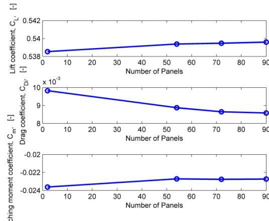
Fig. 9: Grid convergence history for the Bombardier Dash-8, number of panels in the geometry. Convergence criterion: iteration delta < 0.01.
