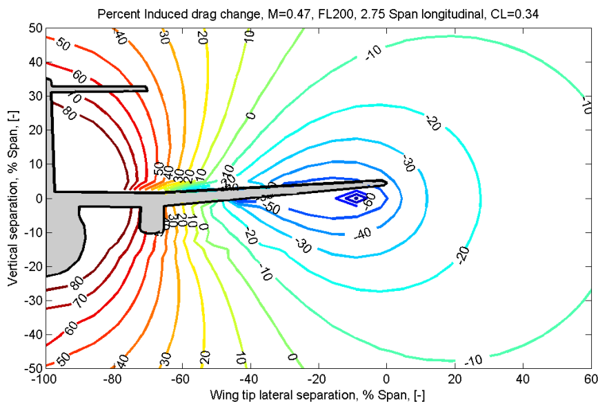
Fig. 10: Iso curves of induced drag reduction in percent of the following aircraft, showing the Bombardier Dash-8 outline. Origin position marks wingtip to wingtip
