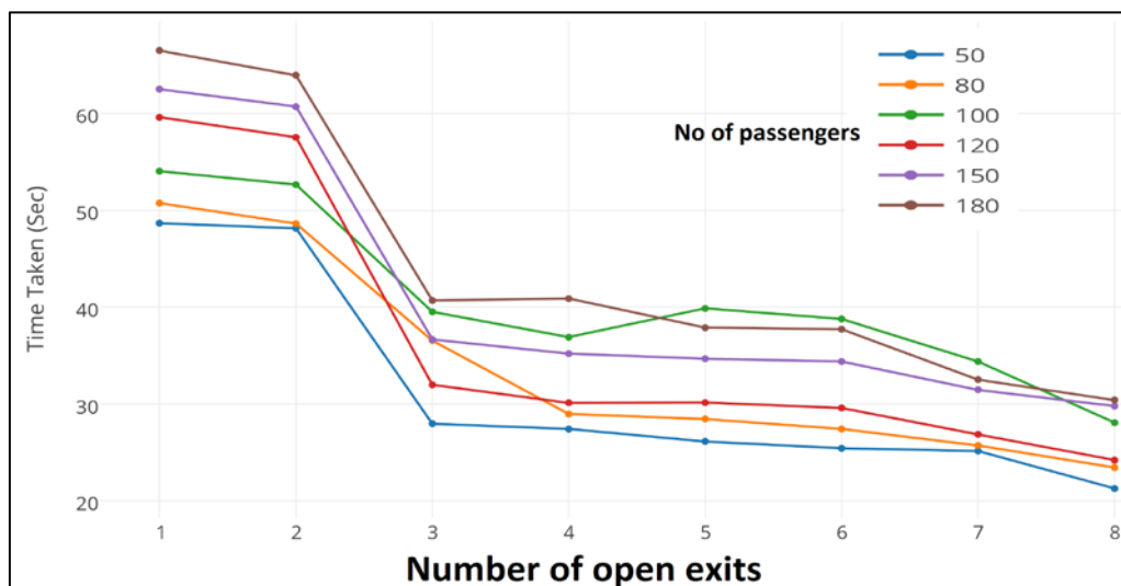
Figure 8: Number of Gates open vs time taken to evacuate
