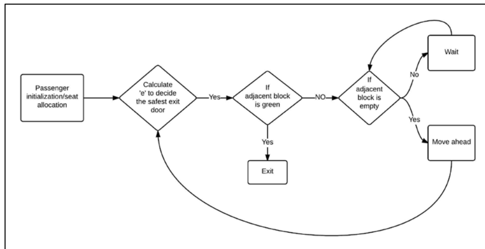
Figure 4: Flowchart of our Computational Algorithm
