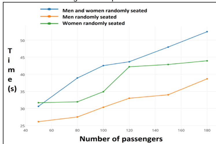
Figure 7: Number of Passengers Vs Time taken to evacuate
