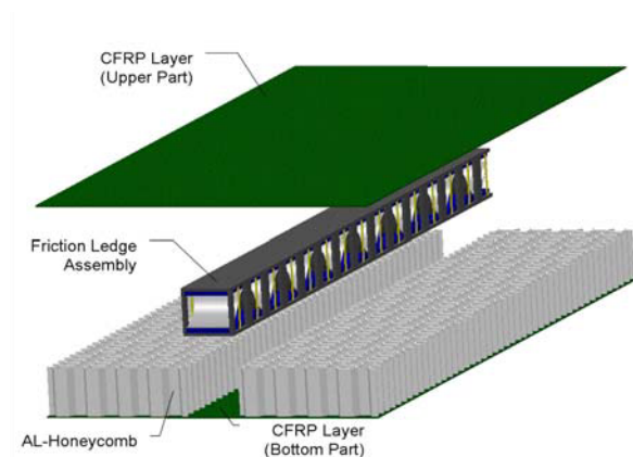
Fig 7: Damping assembly within S/W panel
