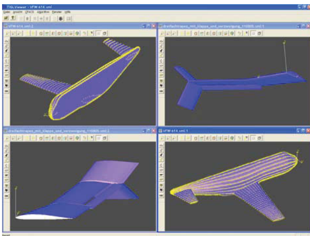
Figure 5: Screenshot showing the visualization of various airplane geometries with the TIGLViewer.
