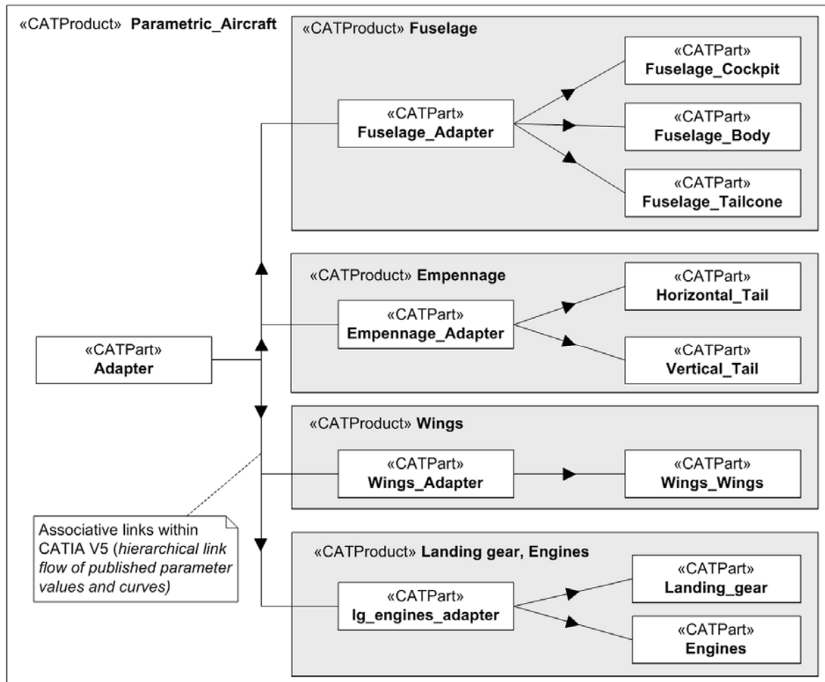
Figure 3: Cascading adapter structure of the parametric aircraft model
