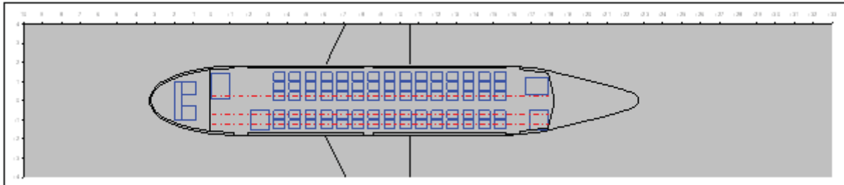
Figure 5: PreSTo cabin floor plan of Fairchild-Dornier 728 re-design
