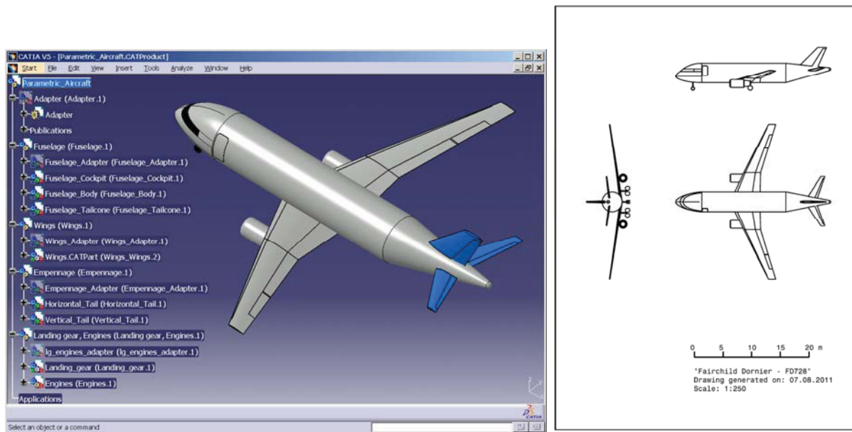
Figure 6: CATIA-model of the FD 728 redesign and the associated three-view drawing
