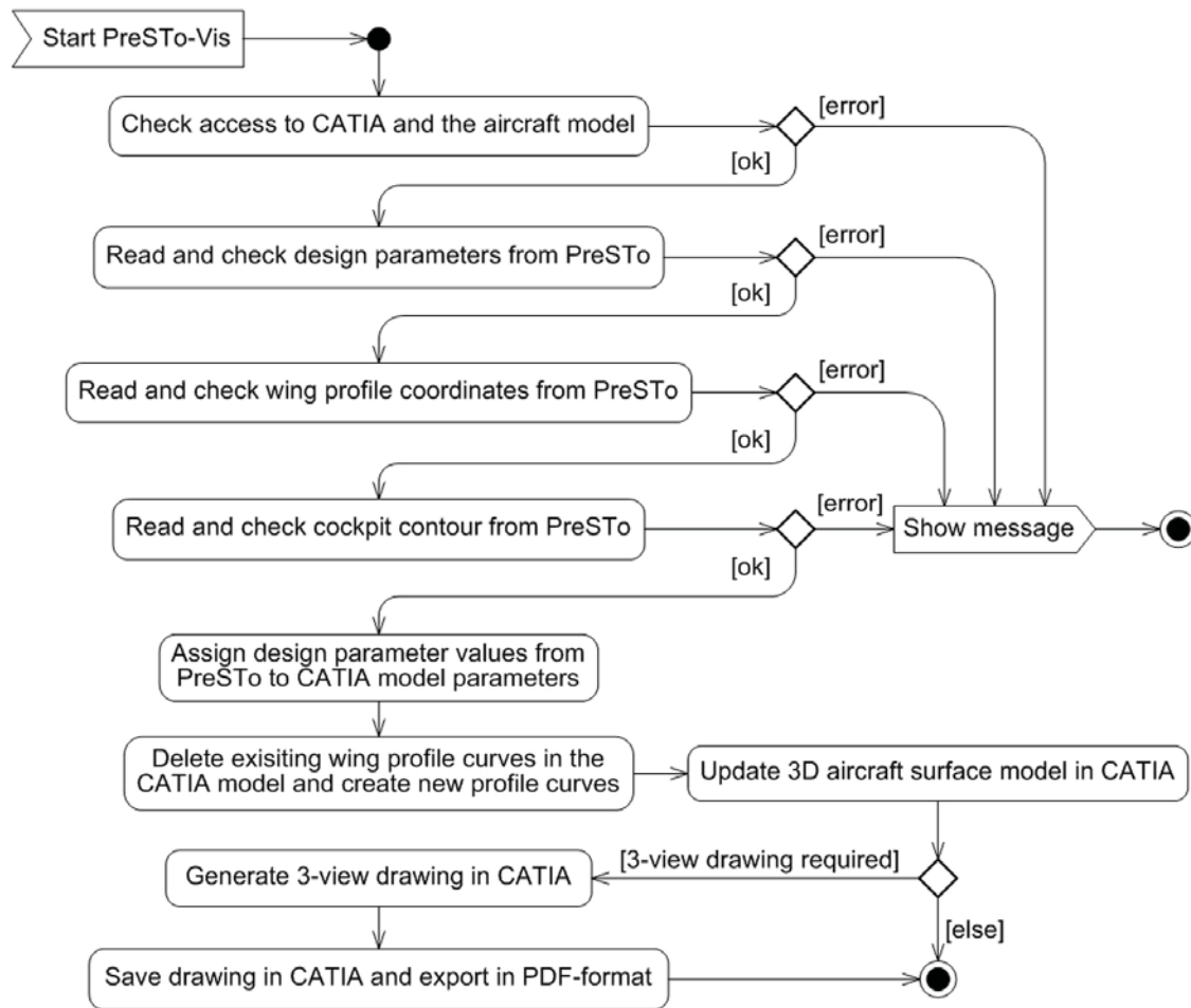
Figure 4: Activity diagram of PreSTo-Vis
