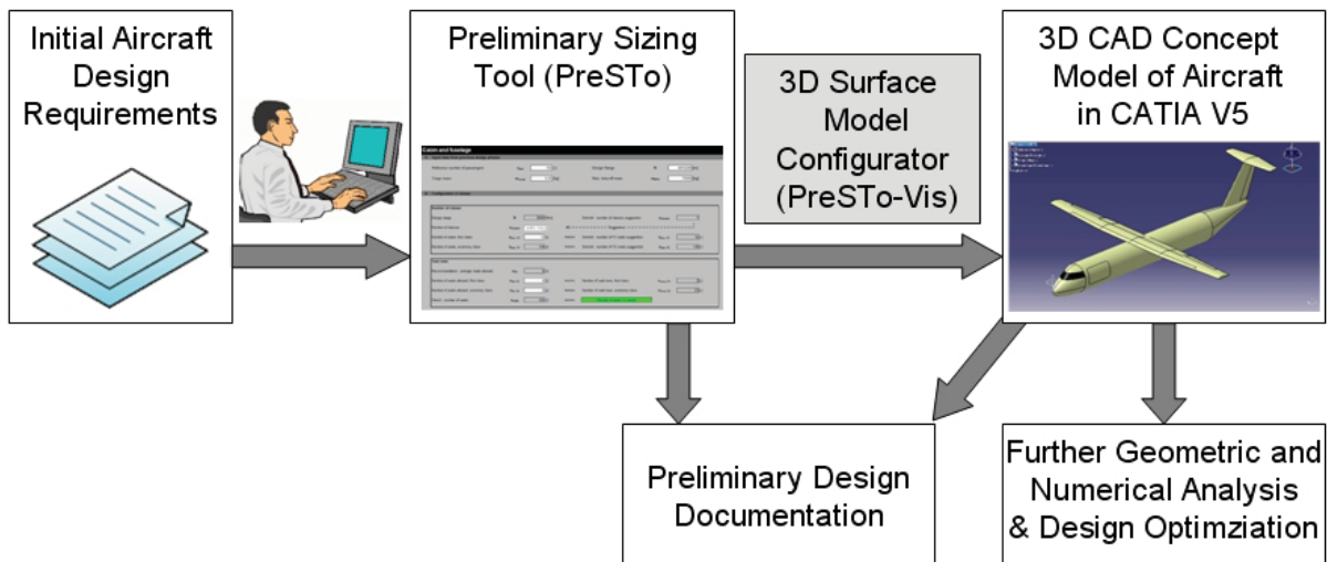
Figure 2: Extension of the preliminary aircraft sizing tool chain by PreSTo-Vis
