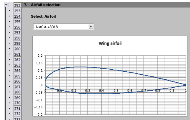
FIG 6. Wing airfoil selection
