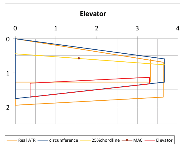
FIG 17. Horizontal tail V01 to real ATR 72
