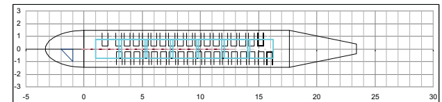
FIG 13. Fuselage top view and floor plan of kerosene versions V01 and V02
