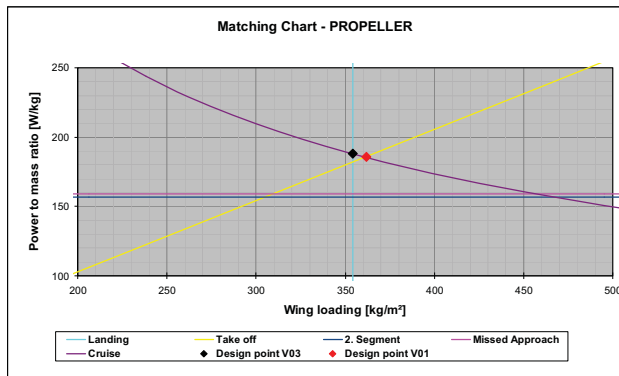
FIG 9. ATR 72 V03 (hydrogen, propeller) matching chart and V01 (kerosene, propeller) design point
