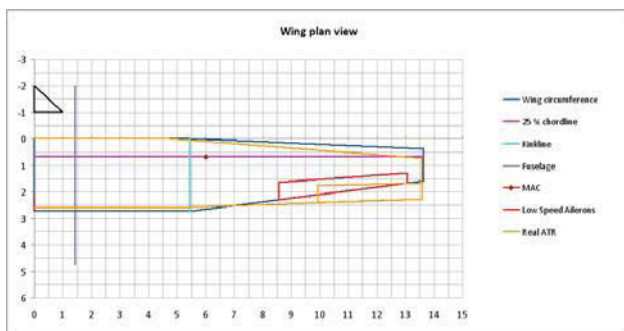
FIG 15. Final PreSTo wing sketch of version V01 including high-lift devices and aileron
