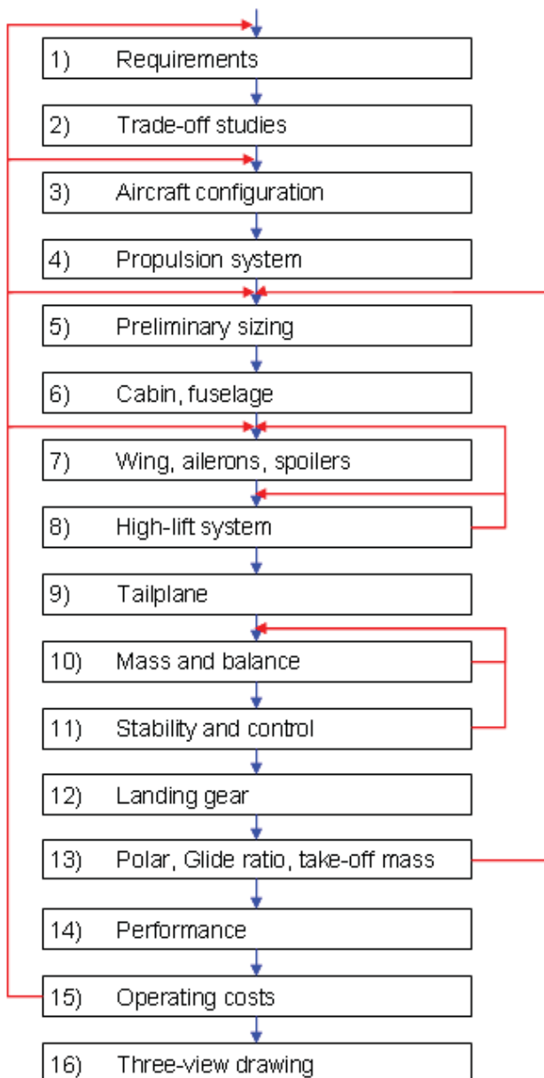
FIG 1. Aircraft design process
