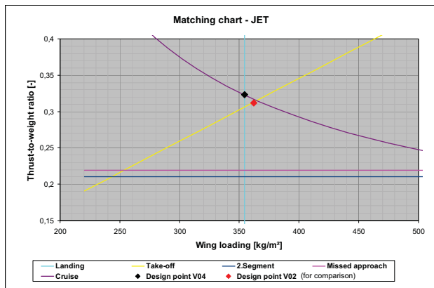
FIG 10. ATR 72 V04 (hydrogen, jet) matching chart and V02 (kerosene, jet) design point
