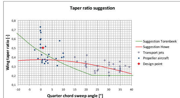
FIG 5. Example parameter suggestion chart (wing taper ratio versus quarter-chord sweep angle)
