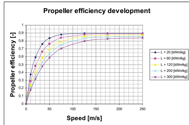
FIG 3. Propeller efficiency development versus airspeed and propeller disc loading
