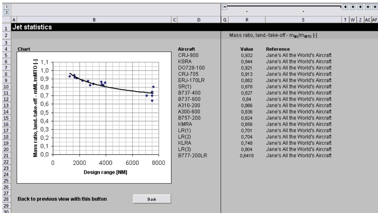
FIG 7. Example statistics chart (ratio of maximum landing to take-off mass versus design range)
