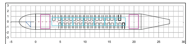
FIG 14. Fuselage top view and floor plan of hydrogen versions V03 and V04
