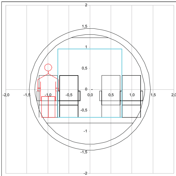
FIG 11. Fuselage cross section
