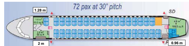
FIG 12. Real ATR 72 floor plan (72 pax)
