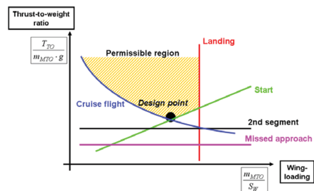
FIG 2. Example of a preliminary sizing matching chart
