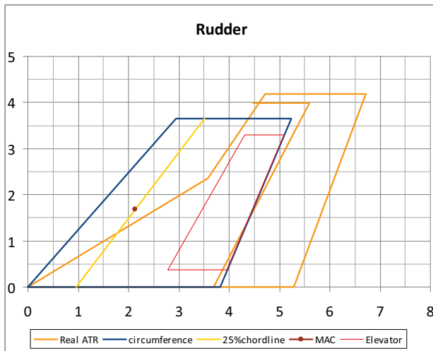
FIG 18. Vertical tail V01 to real ATR 72
