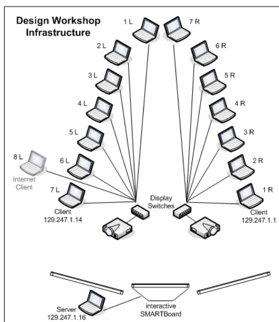
Figure 3: Sketch of Design Workshop at DLR-Bremen as preliminary Concurrent Engineering Facility
