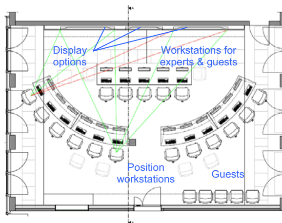
Figure 6: Sketch of Concurrent Engineering Facility of DLR Bremen with 12 special positions and work stations for external experts and guests.
