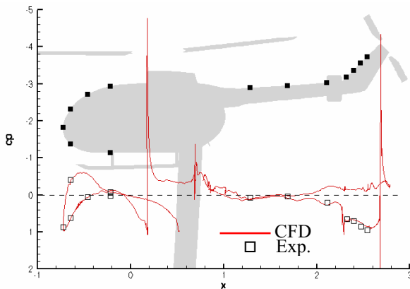
Figure 18 Instantaneous pressure distribution in the mid-section on the fuselage surface ( \psi_{MR}=0 )
