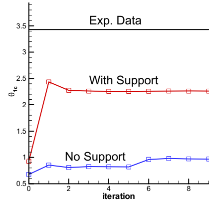
Figure 15 Convergence of longitudinal pitch angle with and without model support
