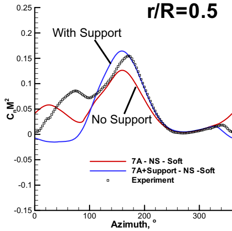
Figure 14 Comparison of lift evolution at mid-span of the blade with and without model support
