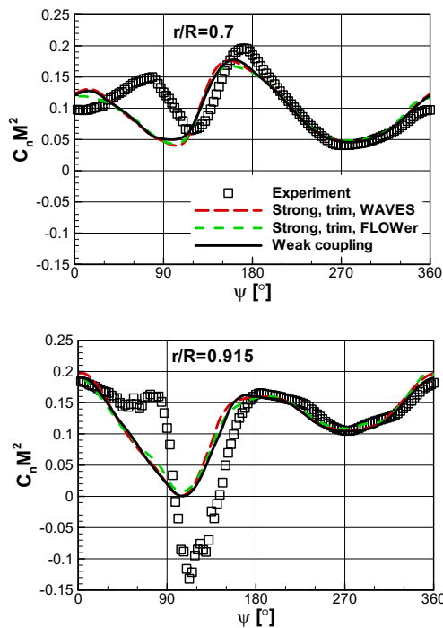
Figure 12 Comparison of weak and strong coupling calculations with experiment (lift)
