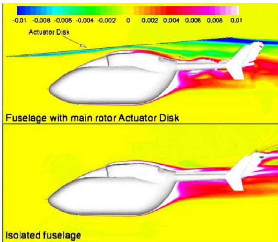
Figure 9 Total Pressure Losses distribution on the middle longitudinal fuselage section, with (upper) and without (lower) AD
