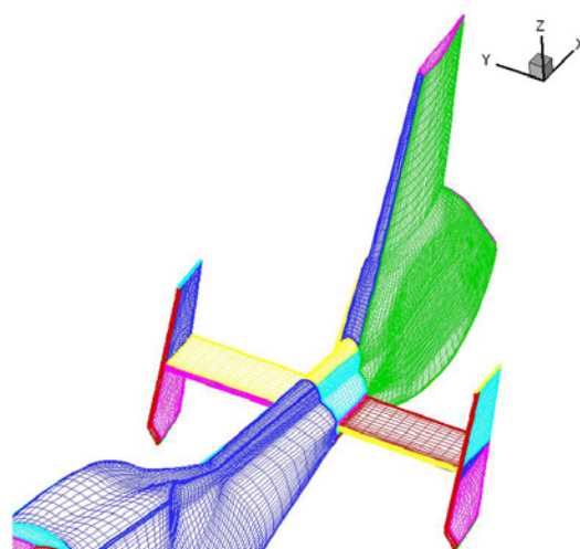
Figure 1 View of the surface grid near the tail
