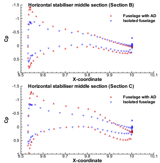
Figure 10 Pressure coefficient distribution on the middle section of the left (Section B) and right (Section C) horizontal stabiliser
