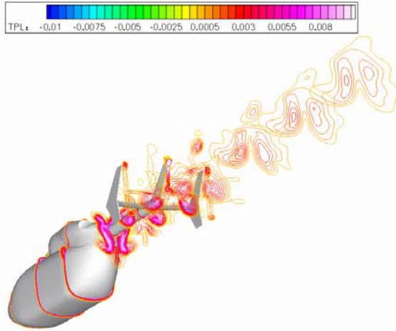
Figure 8 Total Pressure Losses on transversal planes behind the EC145 fuselage at \alpha=0^\circ .
