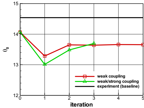
Figure 11 Trim convergence: collective pitch angle
