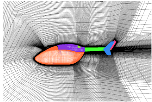
Figure 6 ICEM-Hexa mesh about the EC145 isolated fuselage: middle plane.
