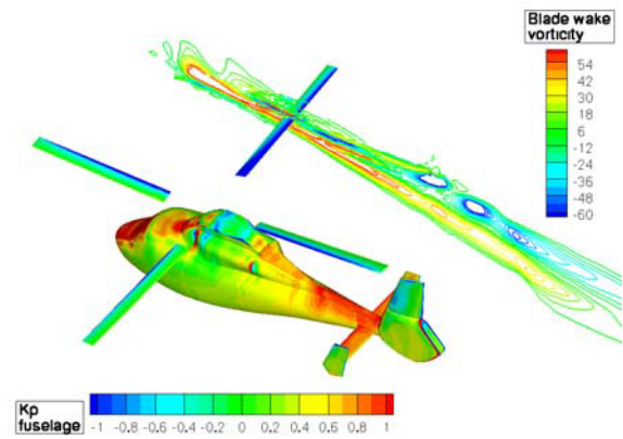
Figure 16 Pressure coefficient on the fuselage surface and vorticity in a section for the Dauphin 365N model in low speed flight
