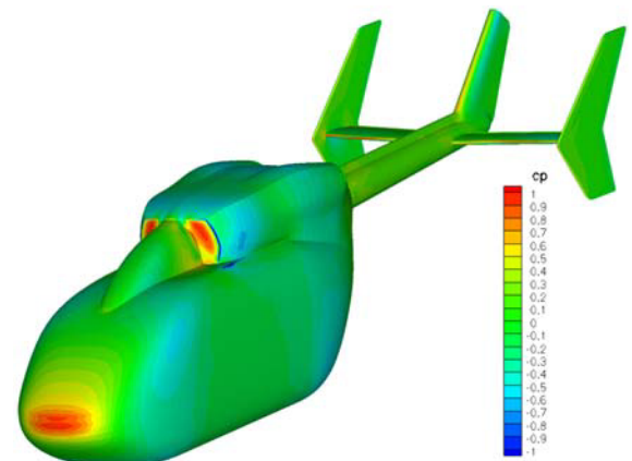
Figure 7 Pressure coefficient distribution on the isolated fuselage of the EC145 helicopter at \alpha=0^\circ .
