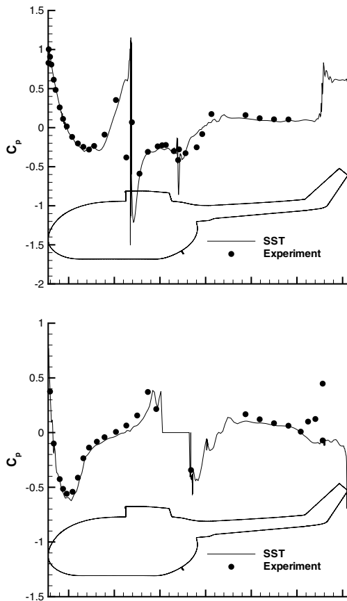
Figure 3 Pressure coefficient at symmetry plane for \alpha = -1.87^\circ (top: upper side, bottom: lower side)
