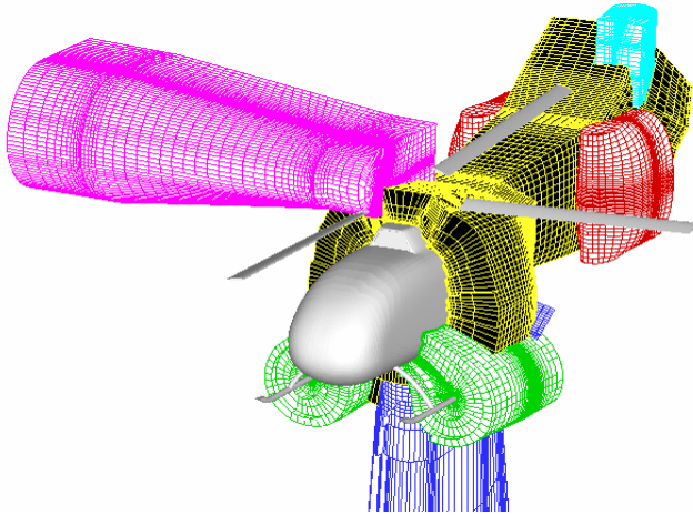
Figure 17 Near-field grids around the BO105 wind tunnel model
