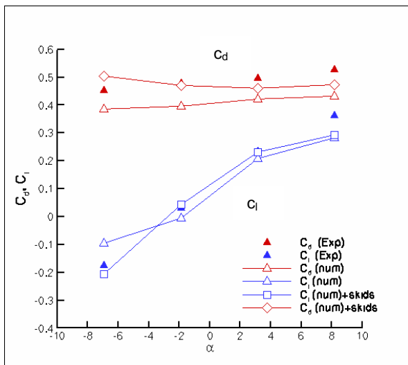
Figure 4 Drag and lift coefficient as a function of pitch angle (BO105)
