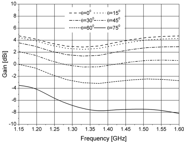
Fig. 6. Element gain over several scan angles simulation.
