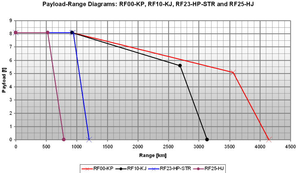
Figure 4.13: Payload-Range Diagrams of RF00-KP, RF10-KJ, RF23-HP-STR and RF25-HJ
