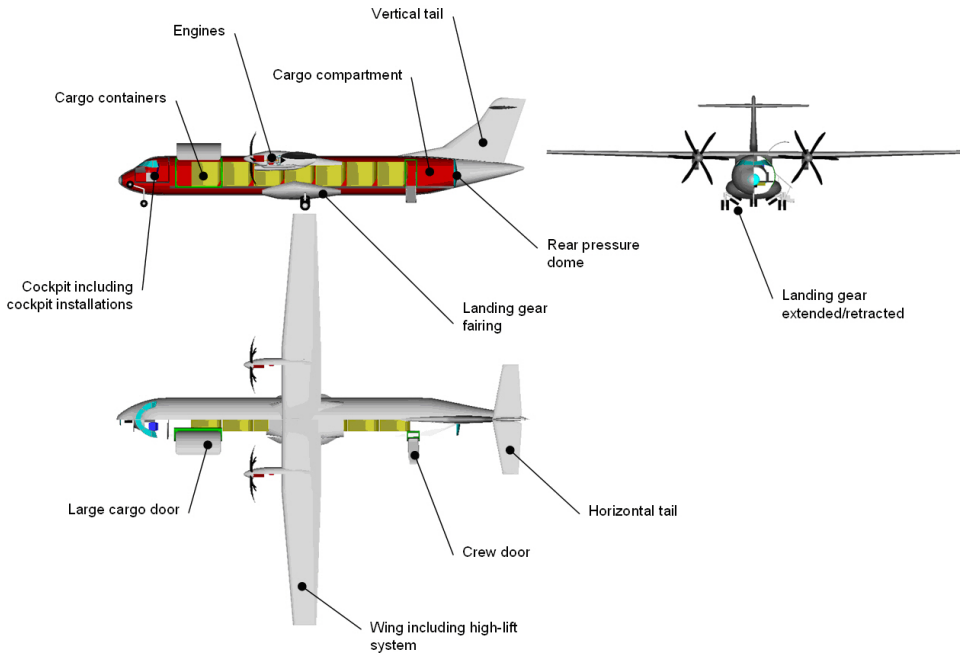
Figure 3.2: Principle PrADO Aircraft Geometry Model
