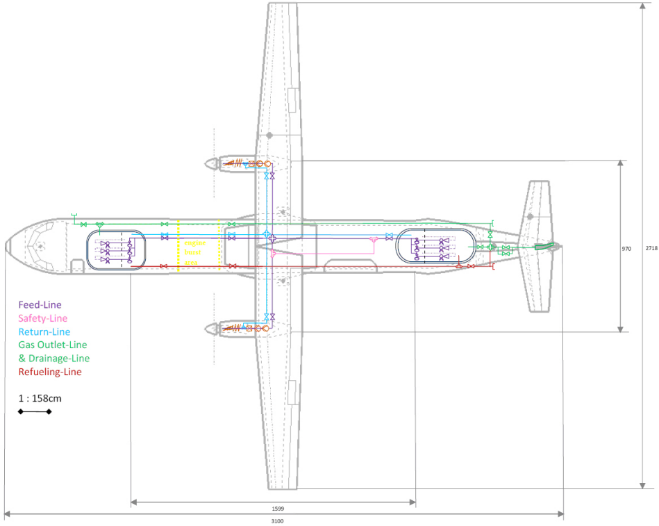
Figure 3.3: Hydrogen Fuel System Layout (Preliminary Version RF20-HP Shown, Batal 2010)
