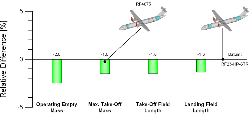
Figure 5.9: Relative Differences in Operating Empty Mass, Max. Take-Off Mass, Take-Off Field Length and Landing Field Length of Version RF4075 to Version RF23-HP-STR
