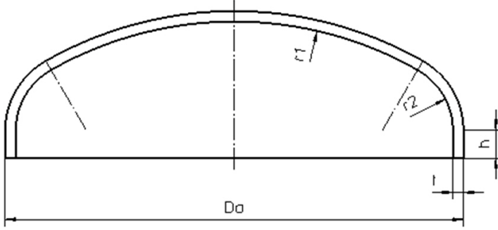
Figure 3.6: Vessel Dished End (wikipedia 2010)
