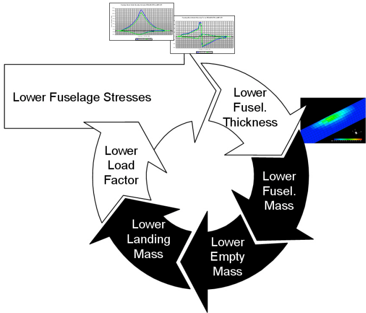
Figure 5.7: Direct Influences and Loop of Snowball Effects of Optimized Wing Position
