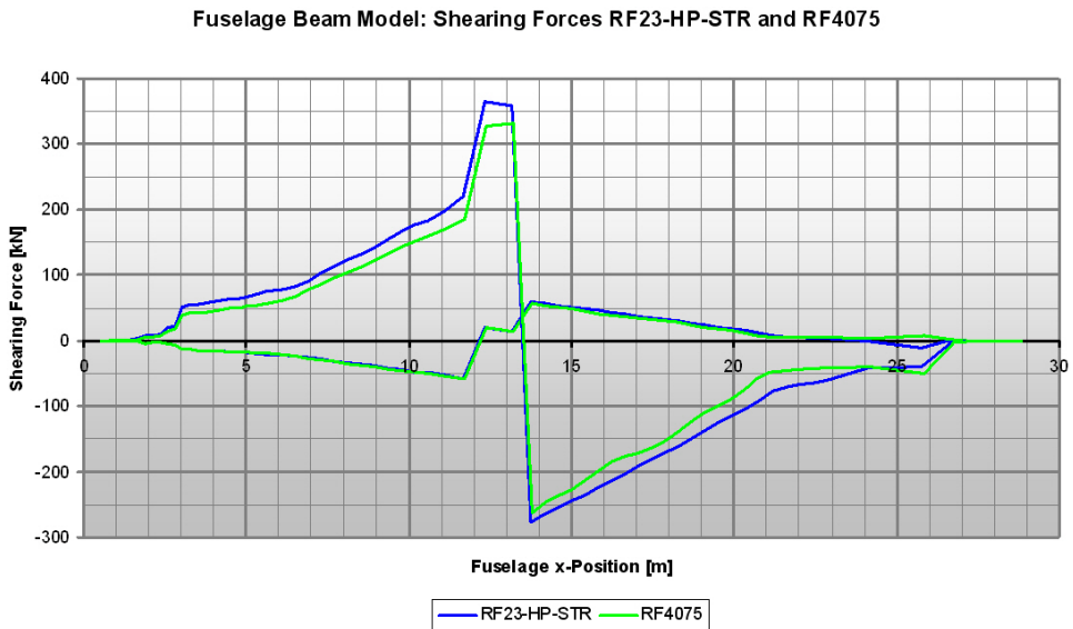
Figure 5.3: Fuselage Beam Model: Shearing Forces of Versions RF23-HP-STR and RF4075
