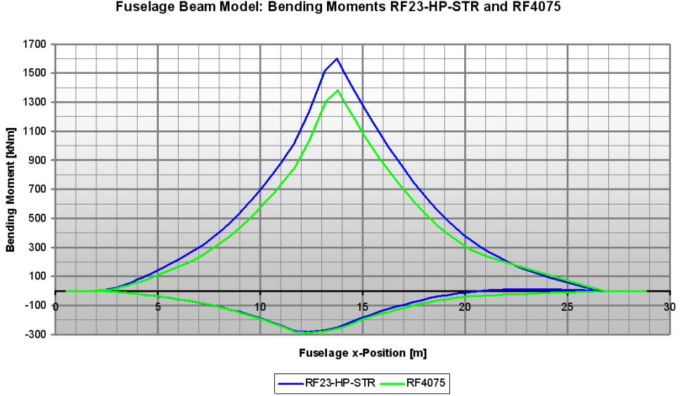
Figure 5.4: Fuselage Beam Model: Bending Moments of Versions RF23-HP-STR and RF4075
