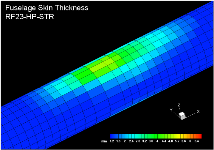
Figure 5.5: Fuselage Skin Thickness of Version RF23-HP-STR
