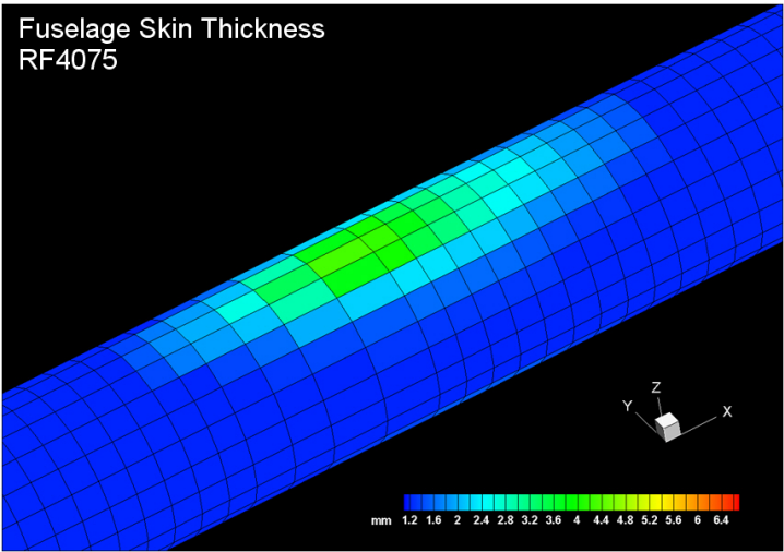
Figure 5.6: Fuselage Skin Thickness of Version RF4075
