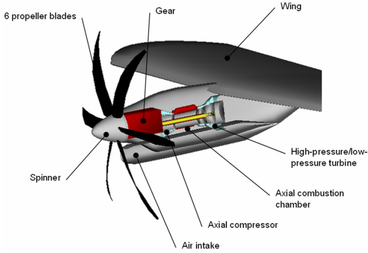
Figure 4.3: PrADO Turboprop Engine Model
