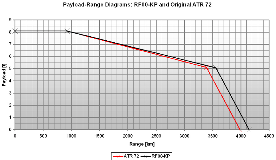
Figure 4.8: Payload-Range Diagrams of RF00-KP and Original ATR 72
