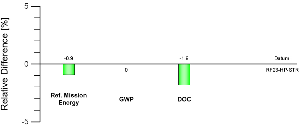
Figure 5.10: Relative Differences in Ref. Mission Energy, GWP and DOC of Version RF4075 to Version RF23-HP-STR
