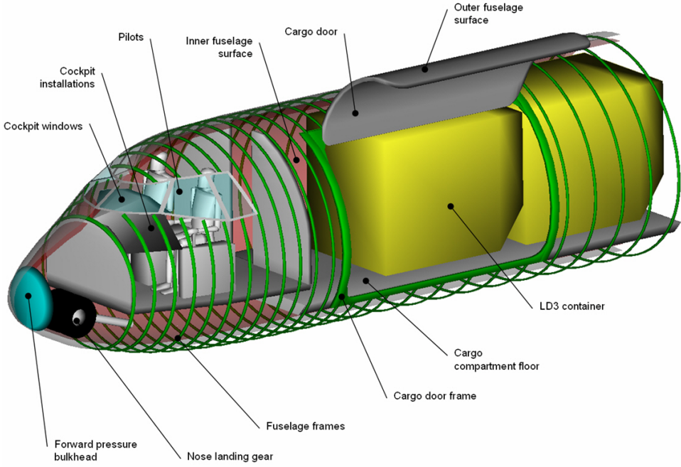
Figure 4.5: Version RF00-KP Forward Fuselage Section
