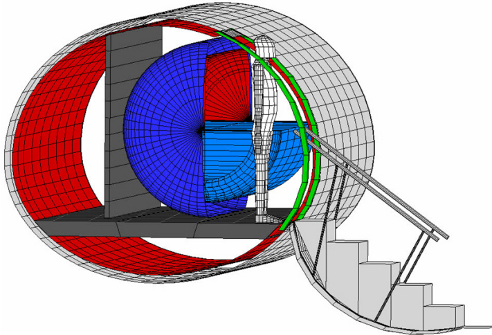
Figure 3.5: Forward Hydrogen Tank Integration (Preliminary Version RF20-HP Shown)
