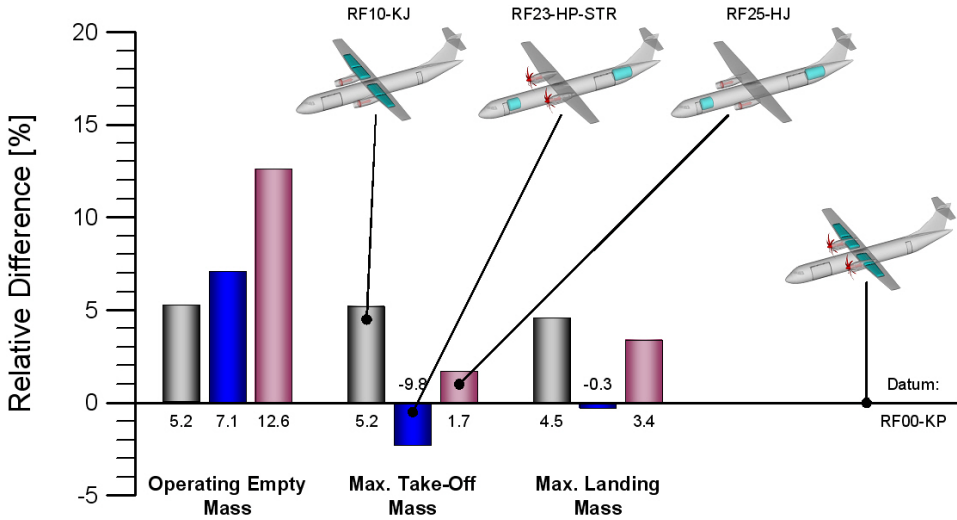
Figure 4.14: Relative Differences in Operating Empty, Max. Take-Off and Max. Landing Mass of Versions RF10-KJ, RF23-HP-STR and RF25-HJ to Reference Version RF00-KP
