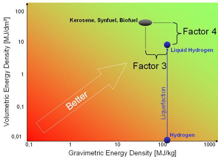
Figure 2.9: Energy Densities of Kerosene and Hydrogen
