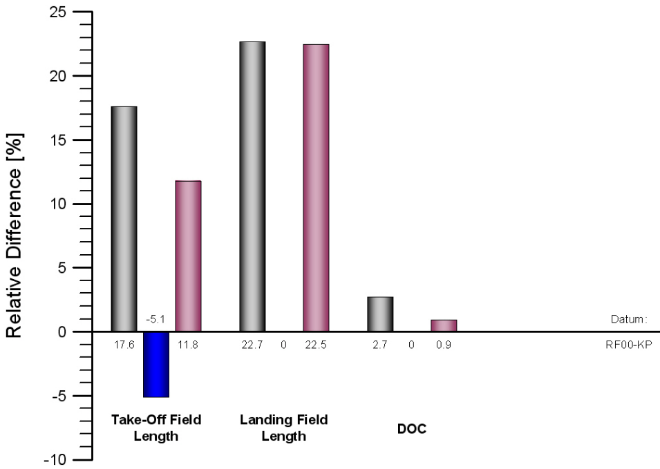
Figure 4.16: Relative Differences in Take-Off Field Length, Landing Field Length and DOC of Versions RF10-KJ, RF23-HP-STR and RF25-HJ to Reference Version RF00-KP
