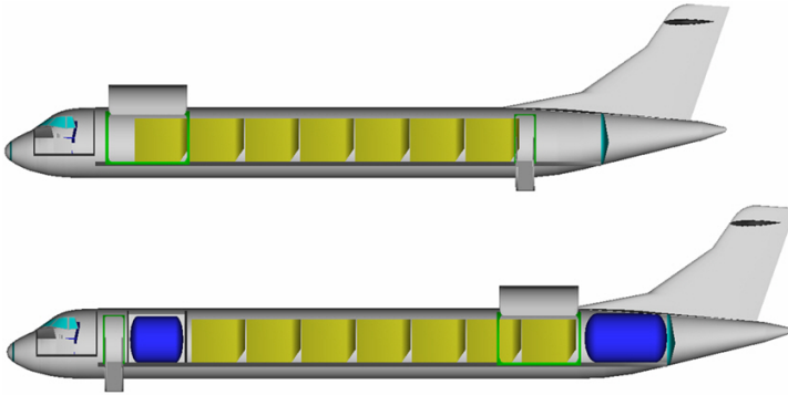
Figure 4.11: Fuselage Comparison of Versions RF00-KP (RF10-KJ) and RF23-HP-STR (RF25-HJ)
