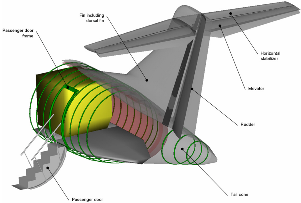
Figure 4.7: Version RF00-KP Tailplane and Rear Fuselage Section
