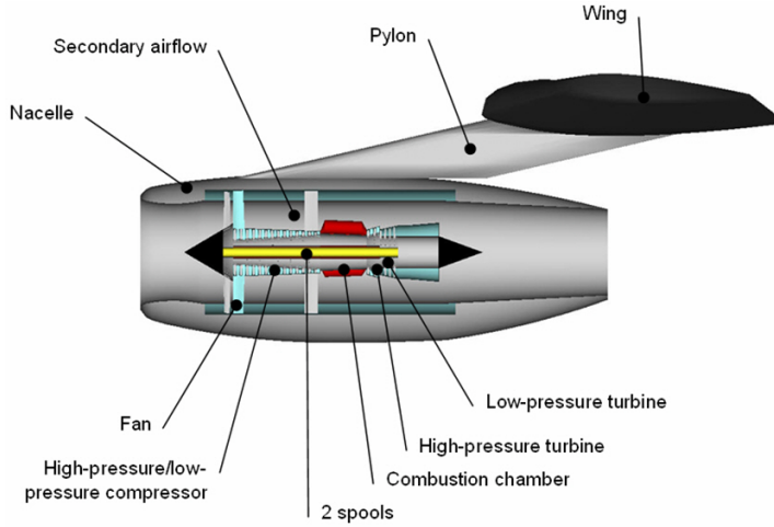
Figure 4.2: PrADO Jet Engine Model
