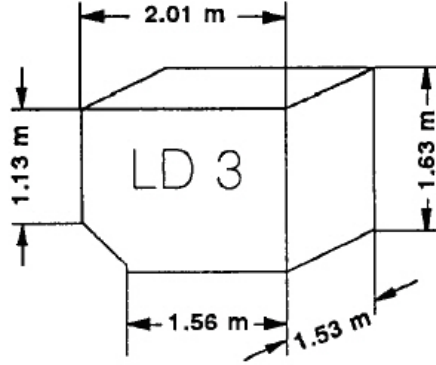
Figure 2.2: LD3 Container Dimensions (Scholz 2005)
