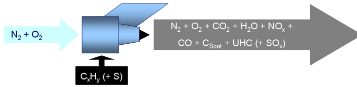
Figure 2.6: Combustion Products of Conventional and Synthetic Kerosene
