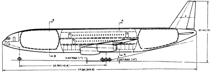
Figure 2.11: Long Range Hydrogen-Fueled Passenger Aircraft (Brewer and Morris 1976)
