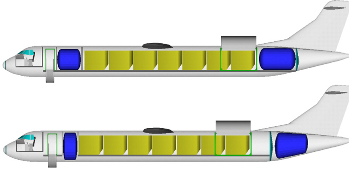
Figure 5.2: Comparison of Fuselages of Versions RF23-HP-STR and RF4075
