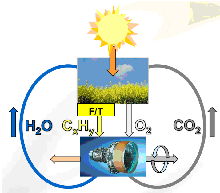
Figure 2.7: Atmospheric Cycles of Hydrogen and Carbon (With Permission of Bauhaus Luftfahrt, Sizmann 2009)
