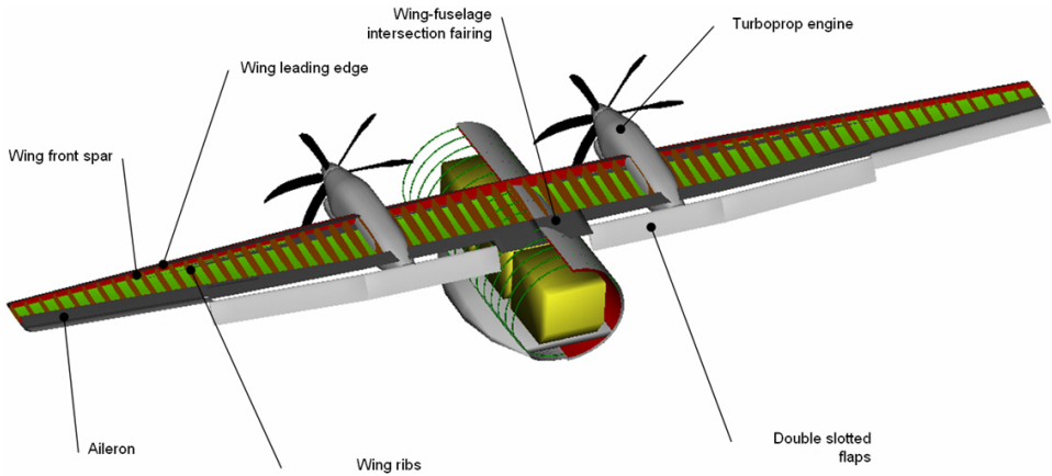
Figure 4.6: Version RF00-KP Wing and Center Fuselage Section
