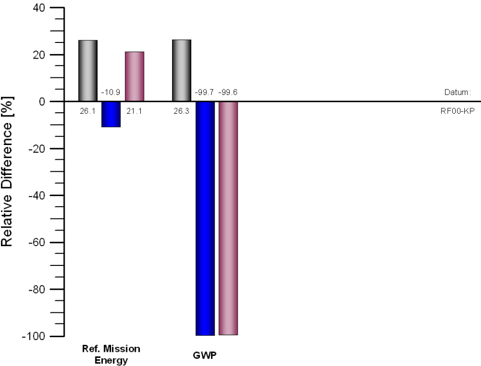
Figure 4.15: Relative Differences in Reference Mission Energy and GWP of Versions RF10-KJ, RF23-HP-STR and RF25-HJ to Reference Version RF00-KP
