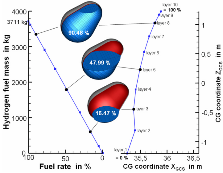
Figure 3.4: PrADO Fuel Mass and Center of Gravity Model (Heinze et al. 2008)
