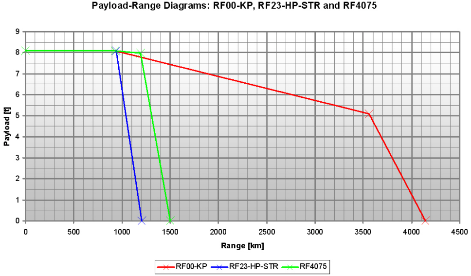
Figure 5.8: Payload-Range Diagrams of RF00-KP, RF23-HP-STR and RF4075
