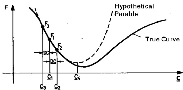
Figure B.1: EXTREM Parabolic Extrapolation (based on Jacob 1982)
