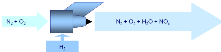
Figure 2.8: Combustion Products of Hydrogen
