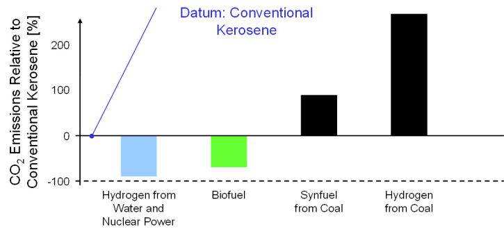
Figure 2.10: Relative CO2 Emissions of Different Fuels (based on IATA 2008)
