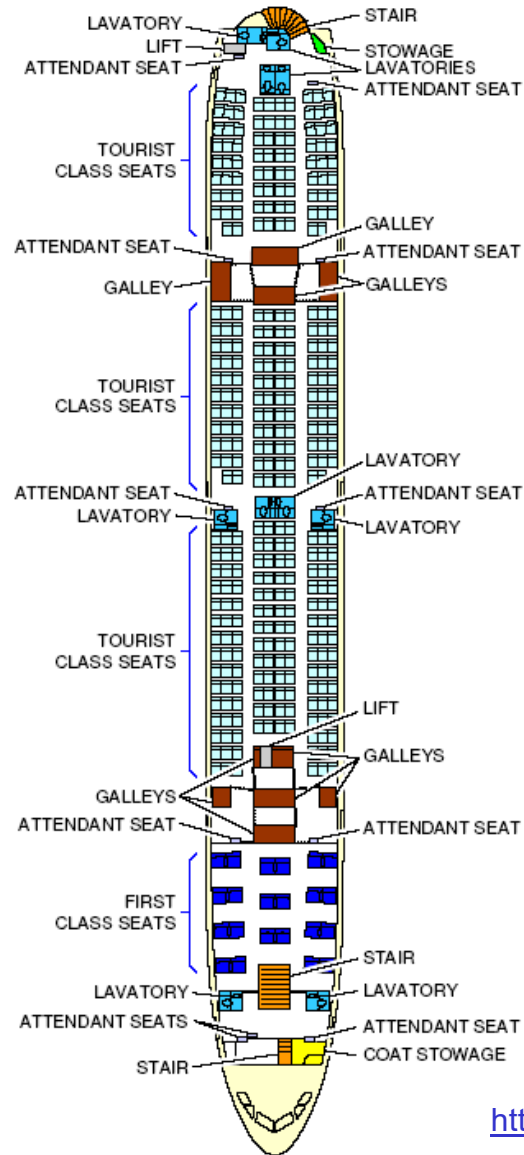
Interior Arrangements - Plan View Standard Configuration - Main Deck
