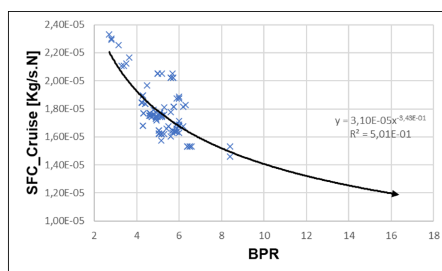
Figure 4: Future trends: SFC improvements with BPR are less pronounced with high BPR. Yes, SFC has been reduced over the decades (by 0.33% p.a.), but this trend is not that clear for all engines.
